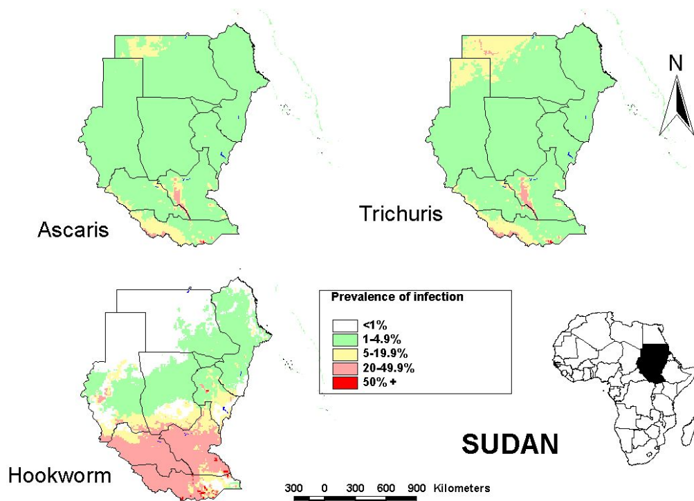
Figure 7: Predicted prevalence of (a) A. lumbricoides , (b) T. trichiura and (c) hookworm in Sudan, based on relationships between observed prevalence of infection in school-aged children and AVHRR satellite & elevation data from the GIS of the US Geological Survey (Brooker et al. 2006)
